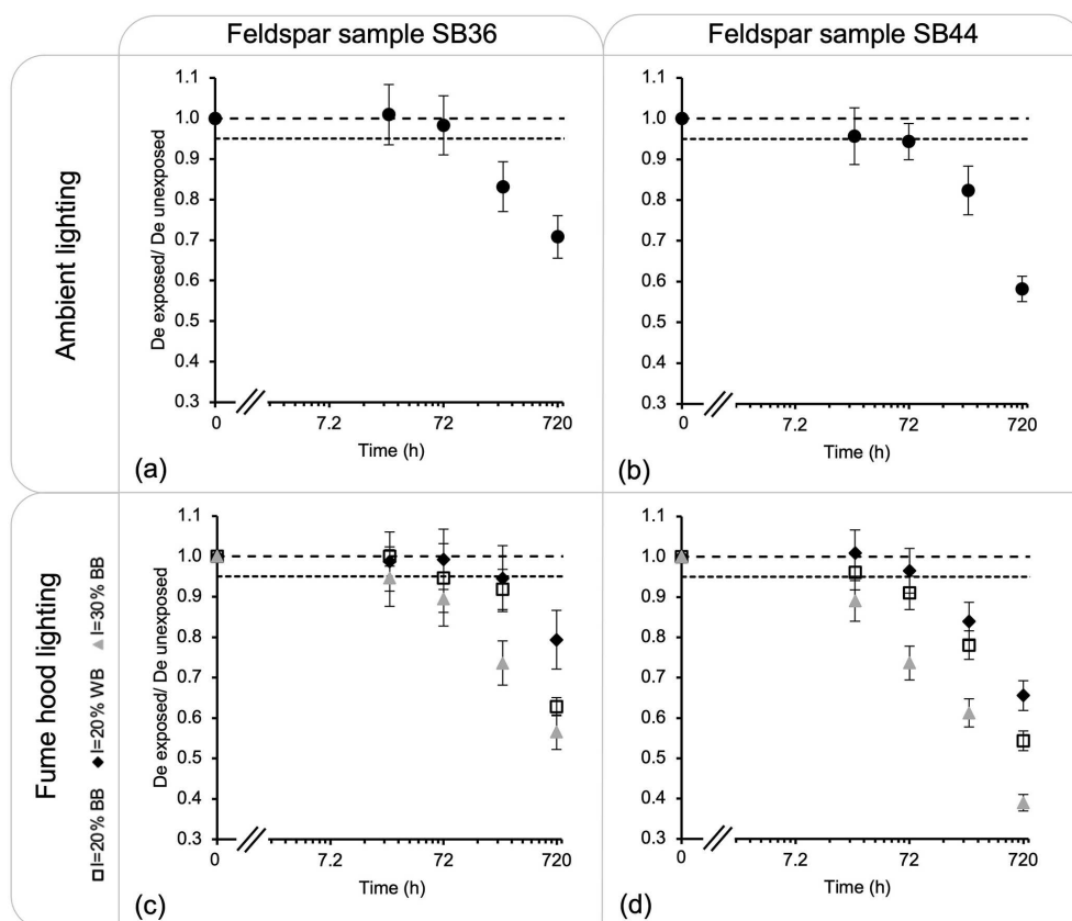
Figure 4. Ratio between the measured IR_{50} dose from aliquots exposed to light and the measured dose from aliquots unexposed. The figures show the results from (a) the feldspar sample SB36 exposed to the ceiling light fixture, (b) the feldspar sample SB44 exposed to the ceiling light fixture, (c) the feldspar sample SB36 exposed to fume hood lighting, and (d) the feldspar sample SB44 exposed to fume hood lighting. Three aliquots were measured per exposure time. The long dashed line indicates a ratio of 1, and the dashed line indicates a loss of 5 %.
